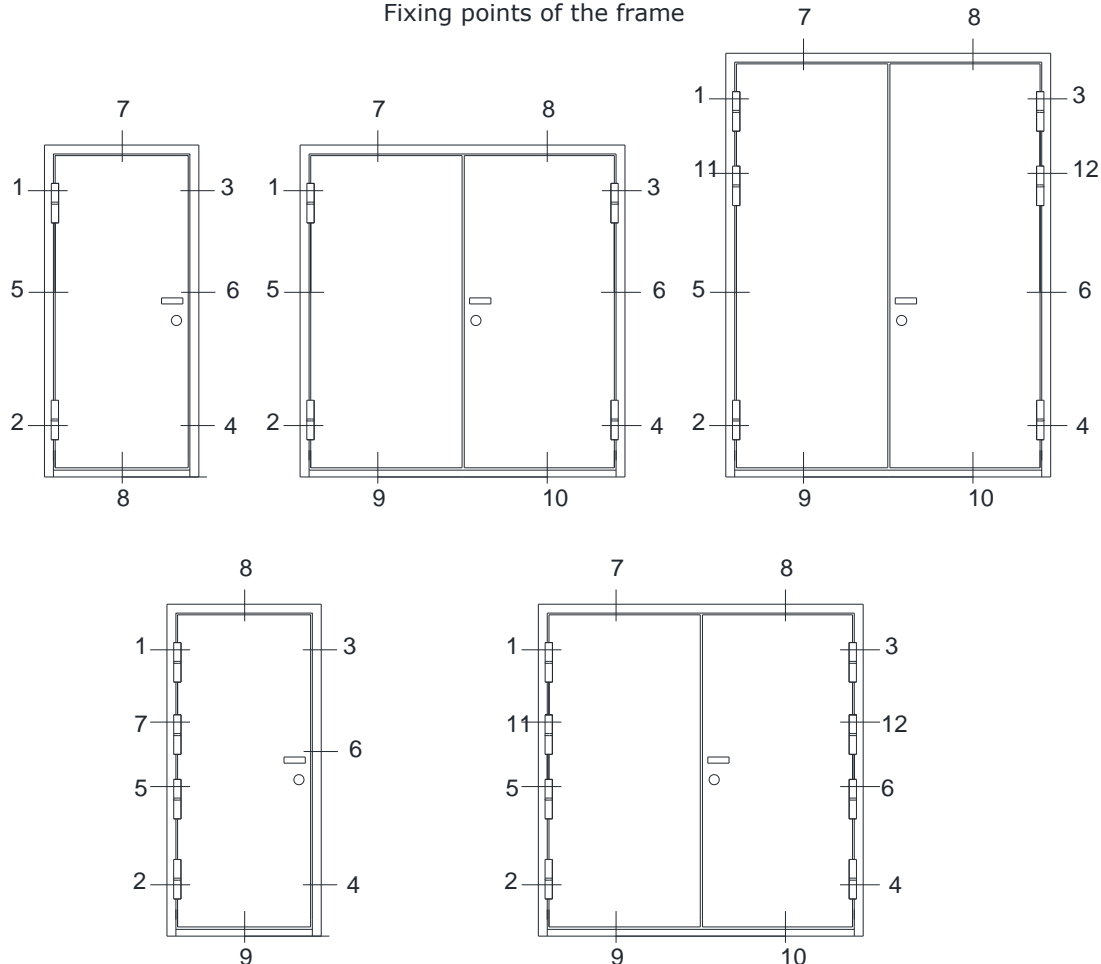
Figure 7. Fixing points of the frame
