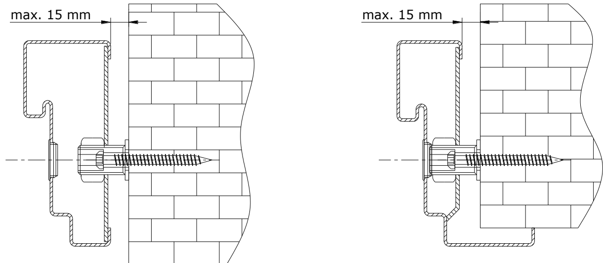
Figure 2. Frame installation with sleeves
