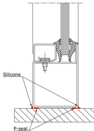
Figure 5 Adding silicone and P-seals
