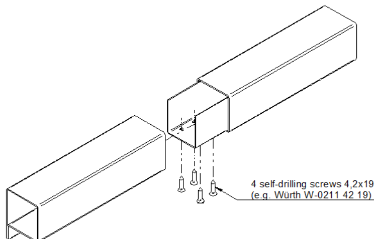
Figure 14 Assembling with connecting profiles
