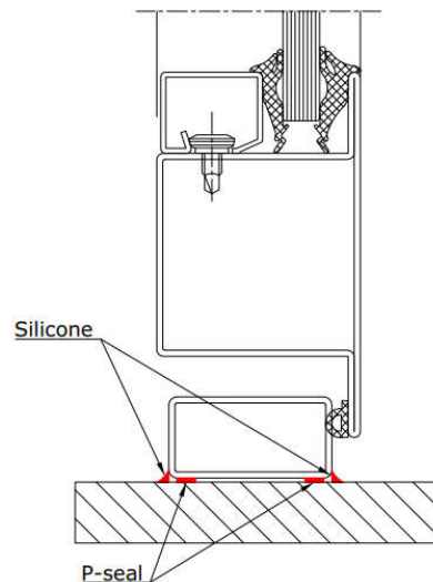
Figure 2 Adding silicone and P-seals
