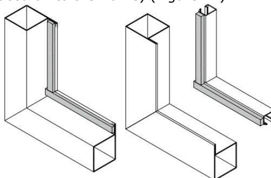
Figure 12 Square shaped seal installation
