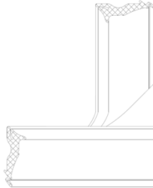
Figure 10 Inner glazing seal installation
