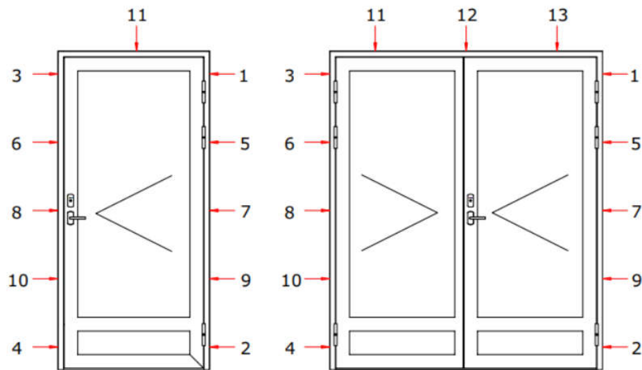
Figure 3 Sequence of fixing points for doors
