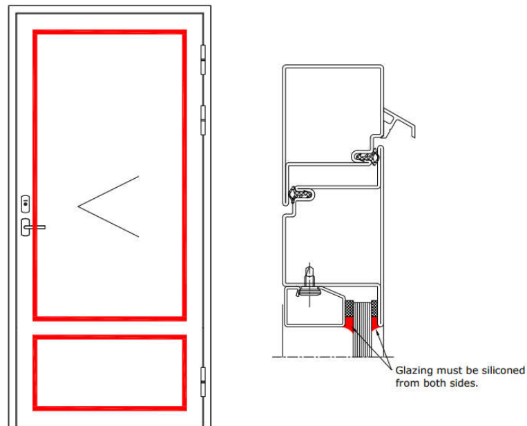
Figure 13 Using silicone for square shaped gaskets.
